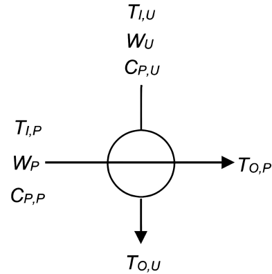
Fig. (2). Heat exchanger.
