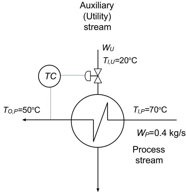
Fig. (6). Heat exchanger for a numerical example.
