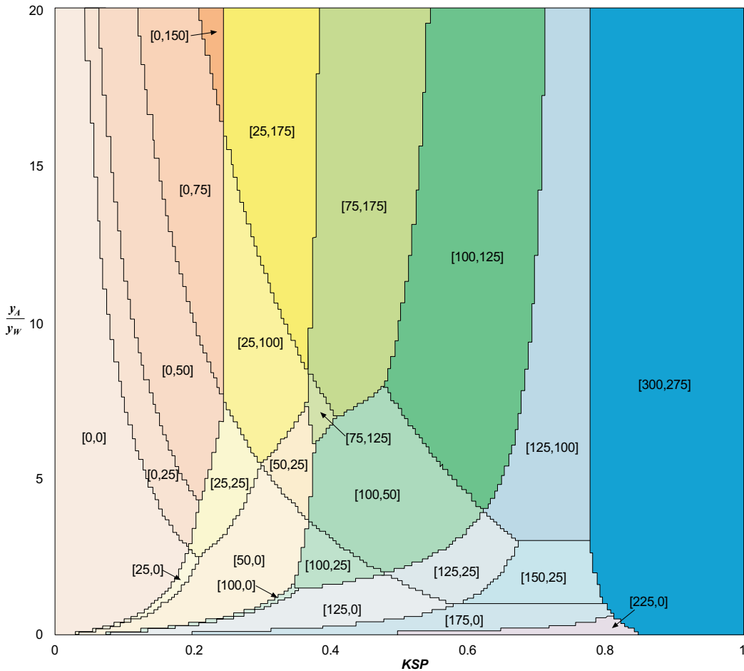
Fig. (10). Recommended designs, shown as [X_A, X_{WU,MAX}] pairs, given k_{SP} and y_A/y_W .
