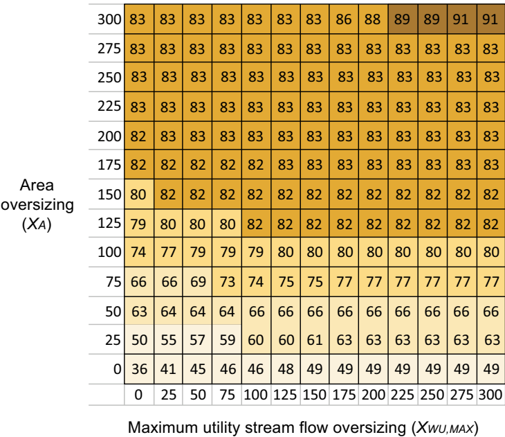
Fig. (9). P(T_{O,P}=T_{O,P}^{SP}) for different values of A and W_{U,MAX} oversizing.
