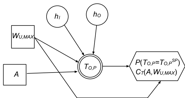
Fig. (4). Influence Diagram for heat exchanger sizing.
