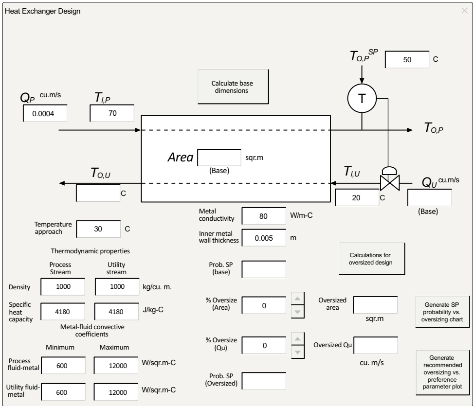
Fig. (12). Main program interface.
