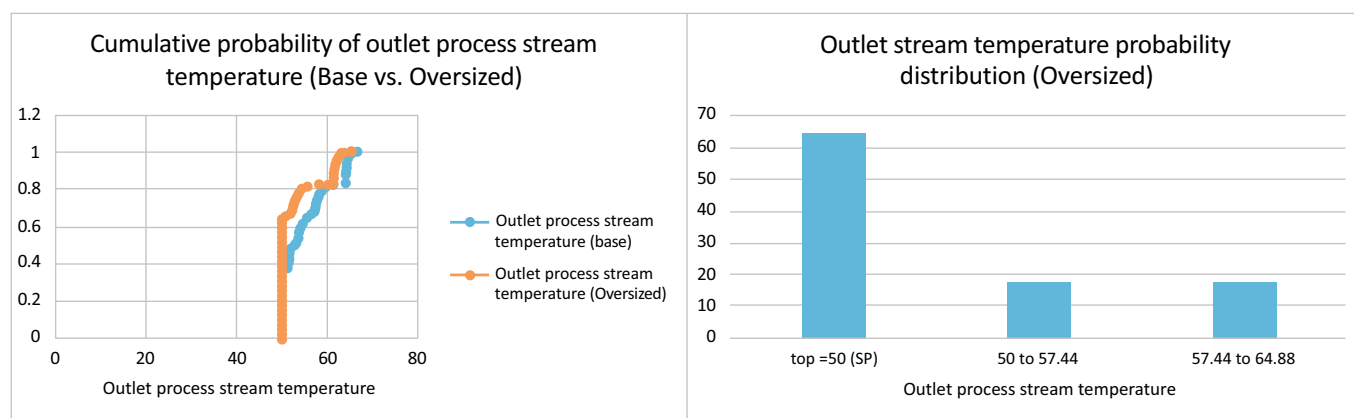
Fig. (15). Program output of oversized design T_{o,p} probability charts.
