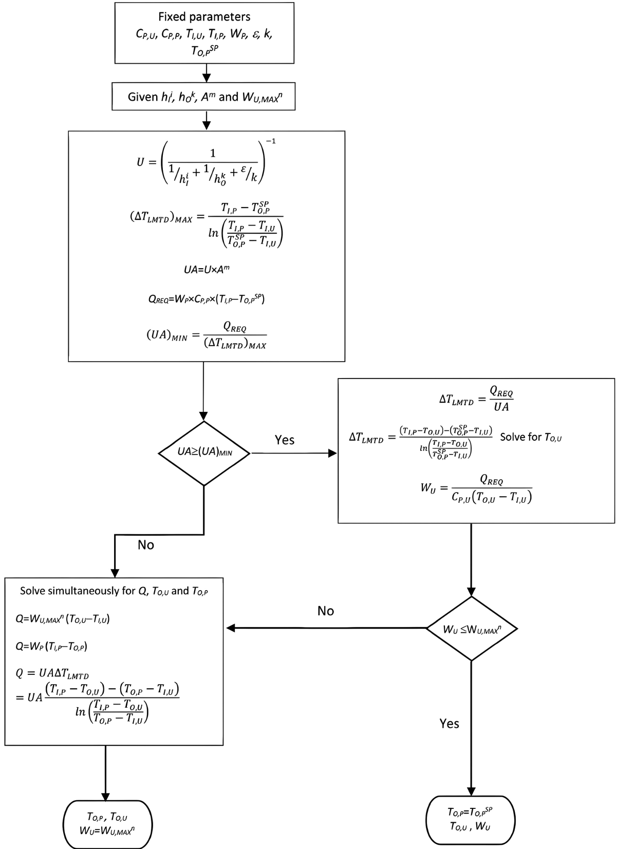
Fig. (5). Algorithm for T_{o,p} and W_U calculation.
