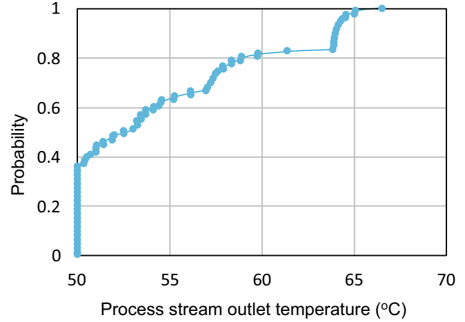
Fig. (7). Cumulative probability distribution of T_{O,P} for the base design.
